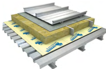
DOUBLE-SKIN METAL ROOF
